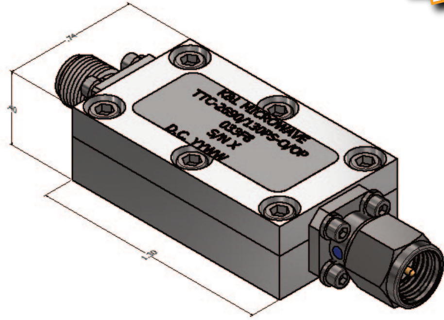
Mechanical Outline
