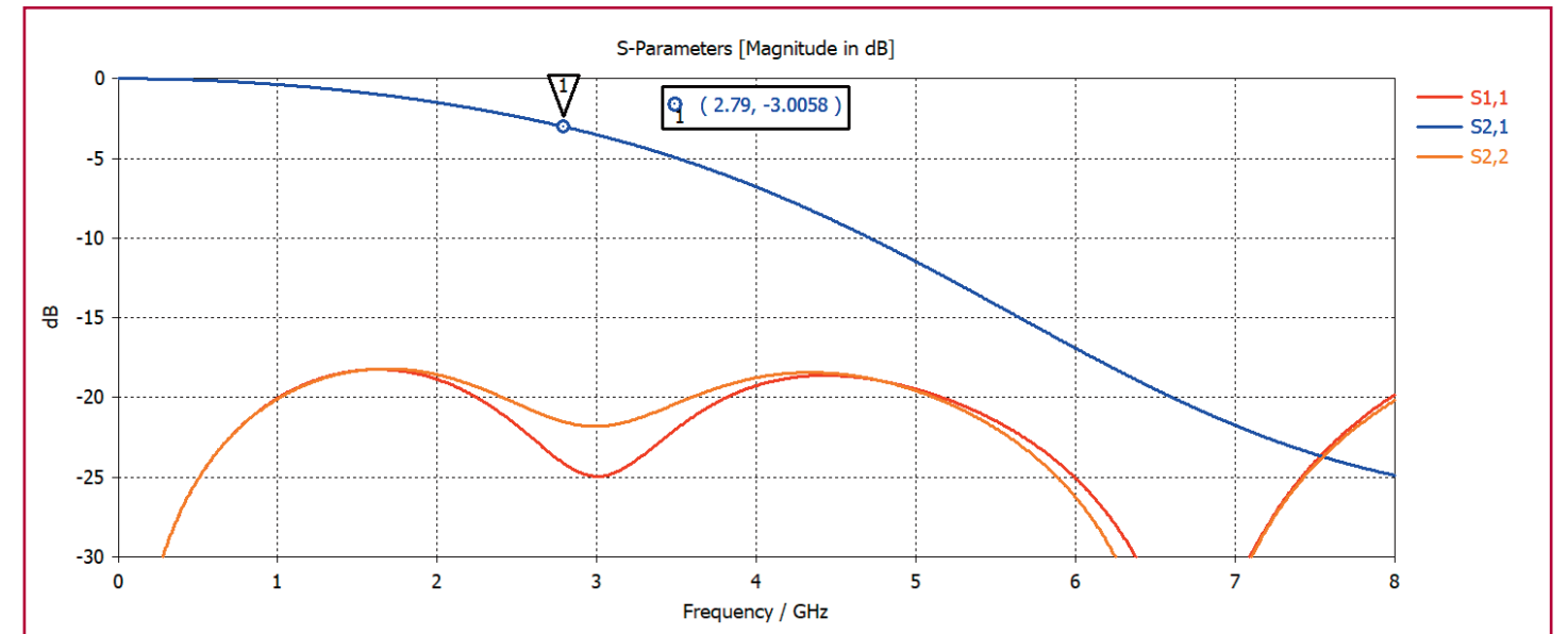
S11, S21, and S22 Response
