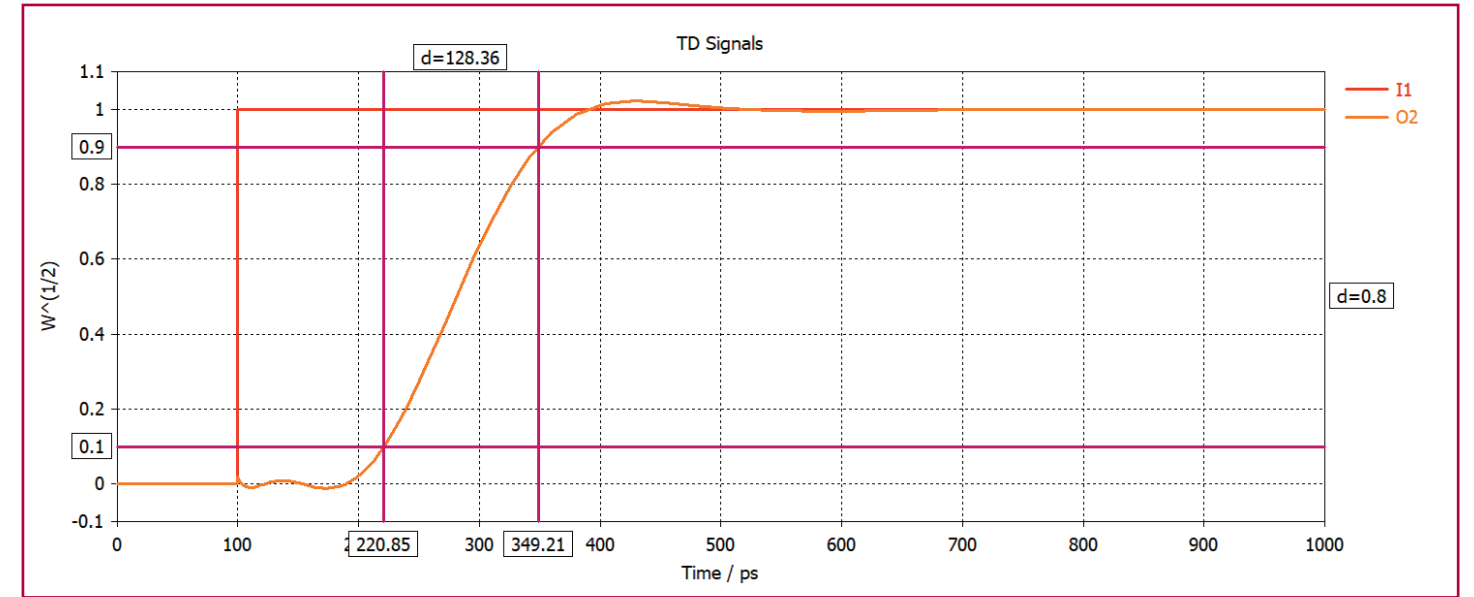
Rise Time of Step Response
