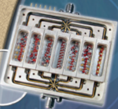
Switched Filter Banks
