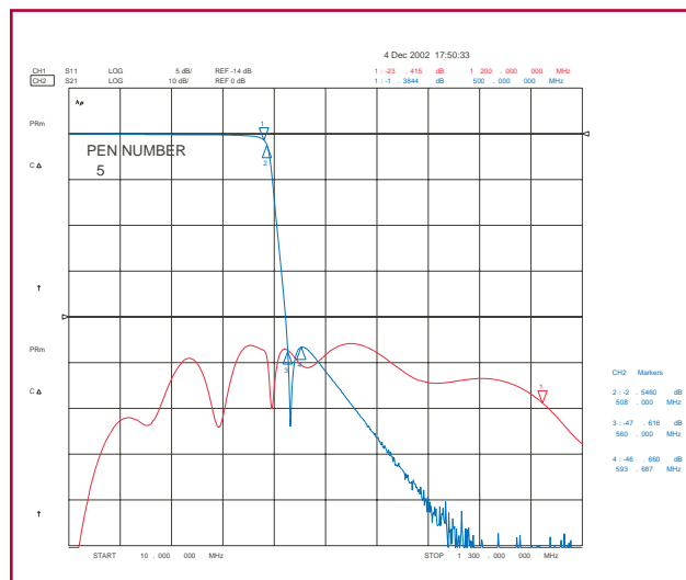
Amplitude Response Channel 1
