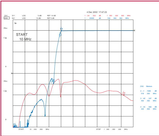
Amplitude Response Channel 2
