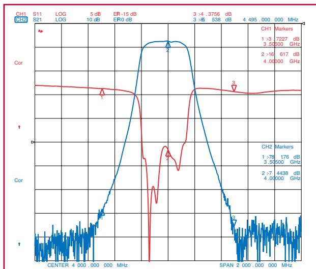
Bandpass Response
