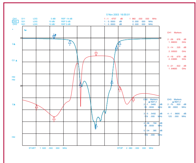
Return Loss
